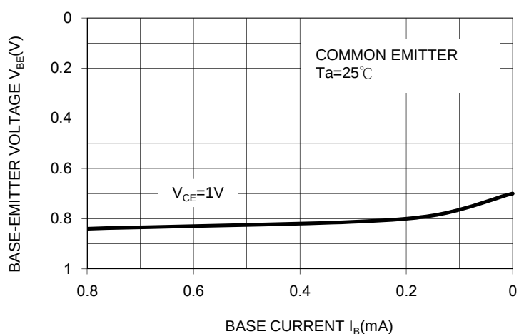
FIG.3 STATIC CHARACTERSTIC
