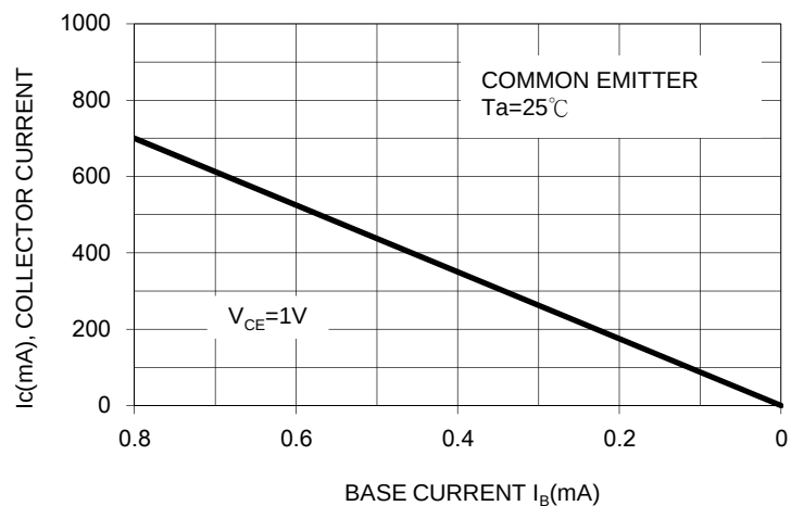
FIG.2 STATIC CHARACTERSTIC
