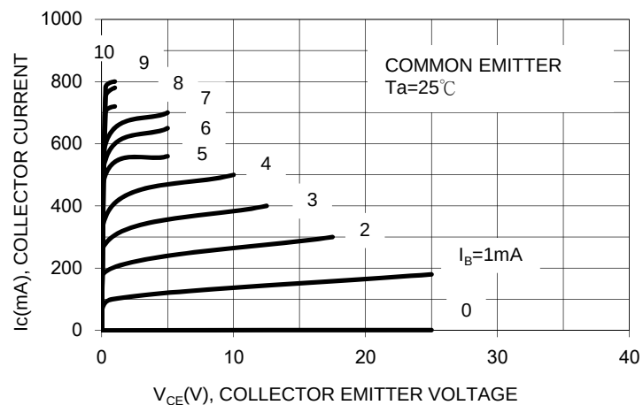
FIG.1 STATIC CHARACTERSTIC
