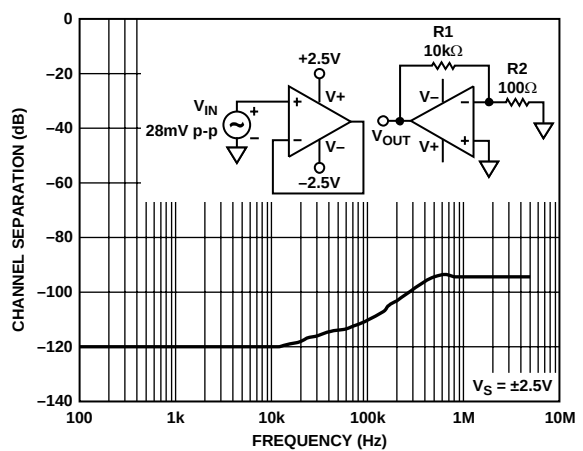
Figure 52. Channel Separation
