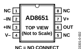
Figure 3. 8-Lead SOIC (R-8)
