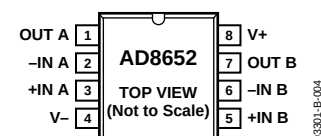
Figure 4. 8-Lead SOIC (R-8)
