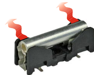
Fig. 5: UL/CSA test with silver tube
