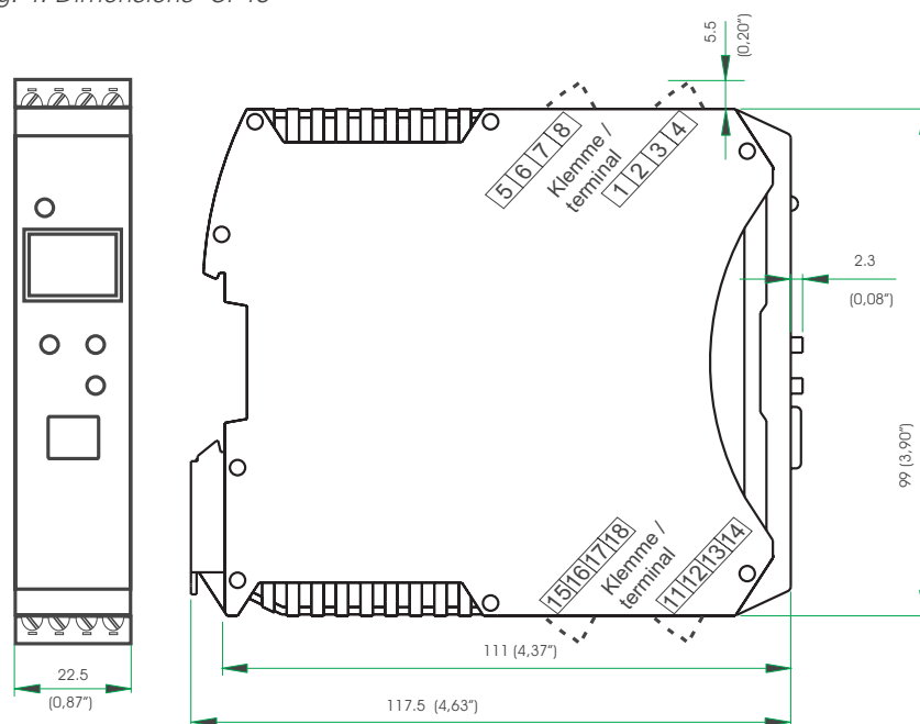
Fig. 4: Dimensions CI 45
