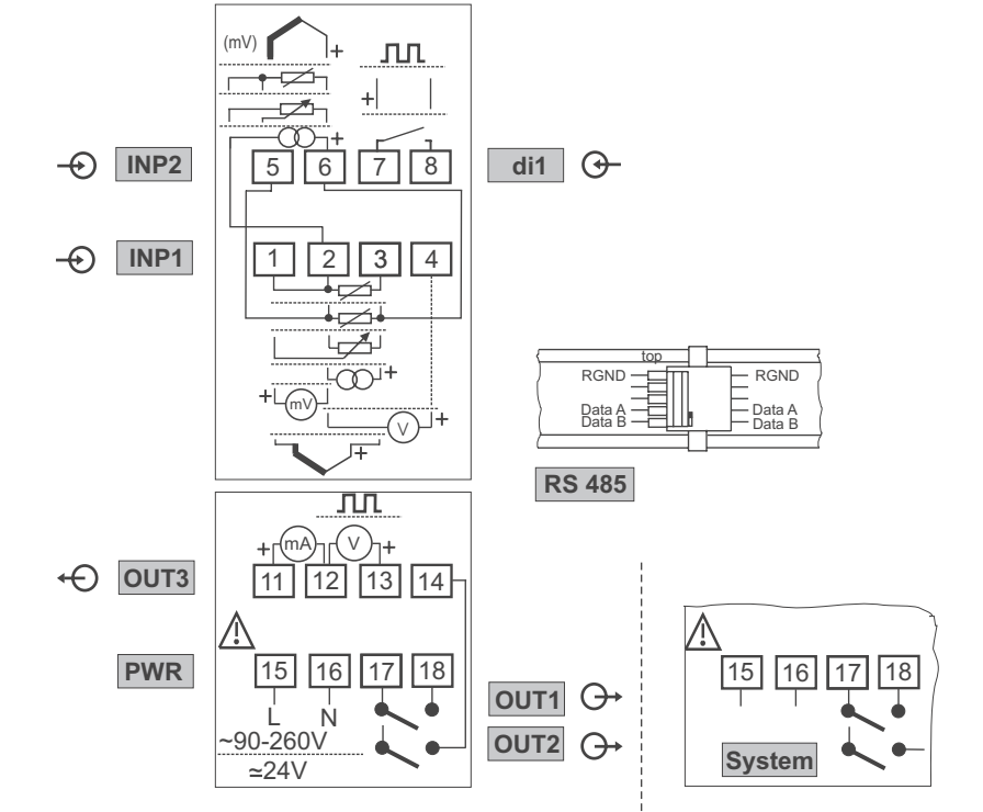
Fig. 2: Connecting diagram CI 45
