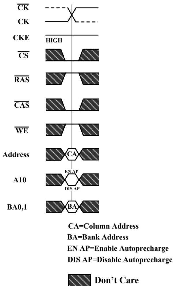
Figure 6. READ Command
