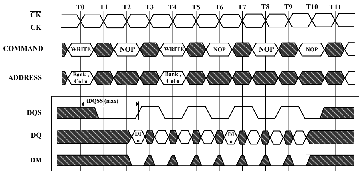
Figure 18. Write to Write Max tDQSS
