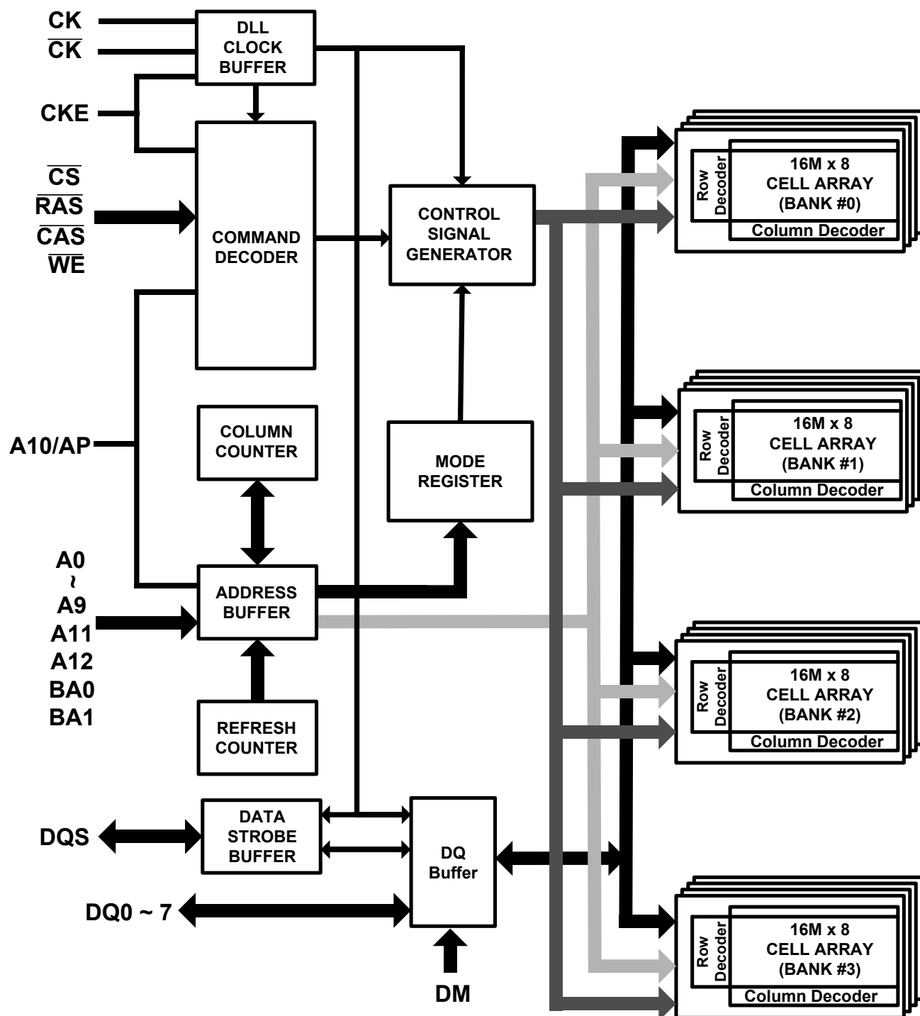
Figure 2. Block Diagram
