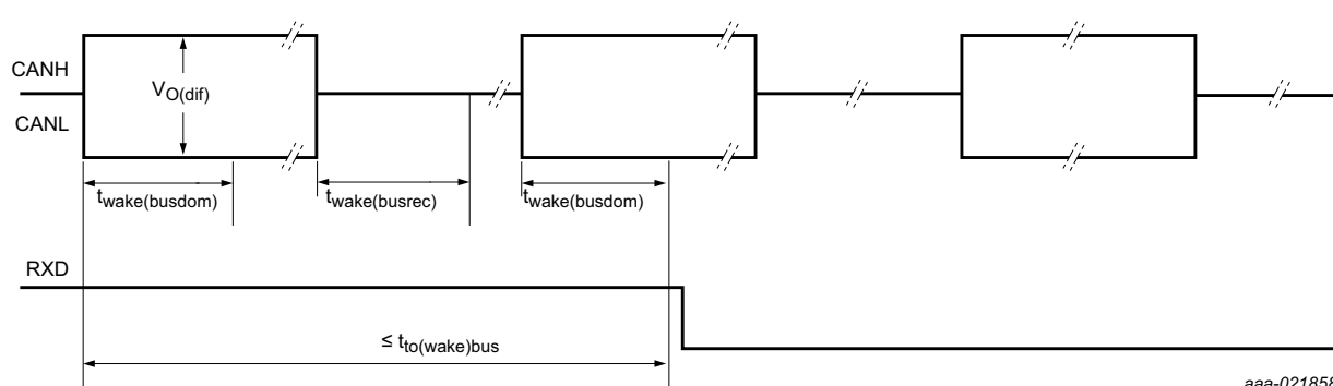
Fig 5. Wake-up timing
