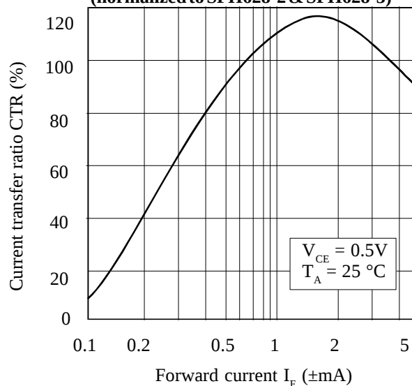
Current Transfer Ratio vs. Forward Current (normalized to SFH628-2 & SFH628-3)
