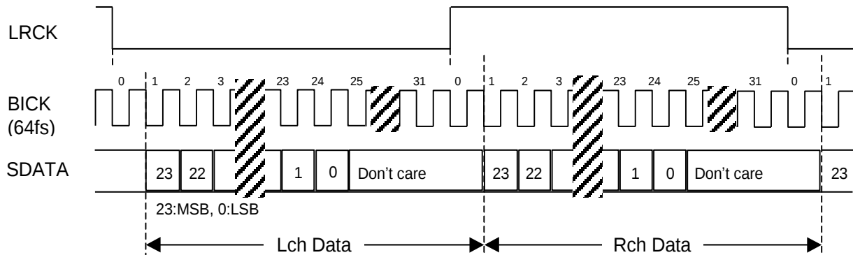
Figure 14. Mode 3 Timing
