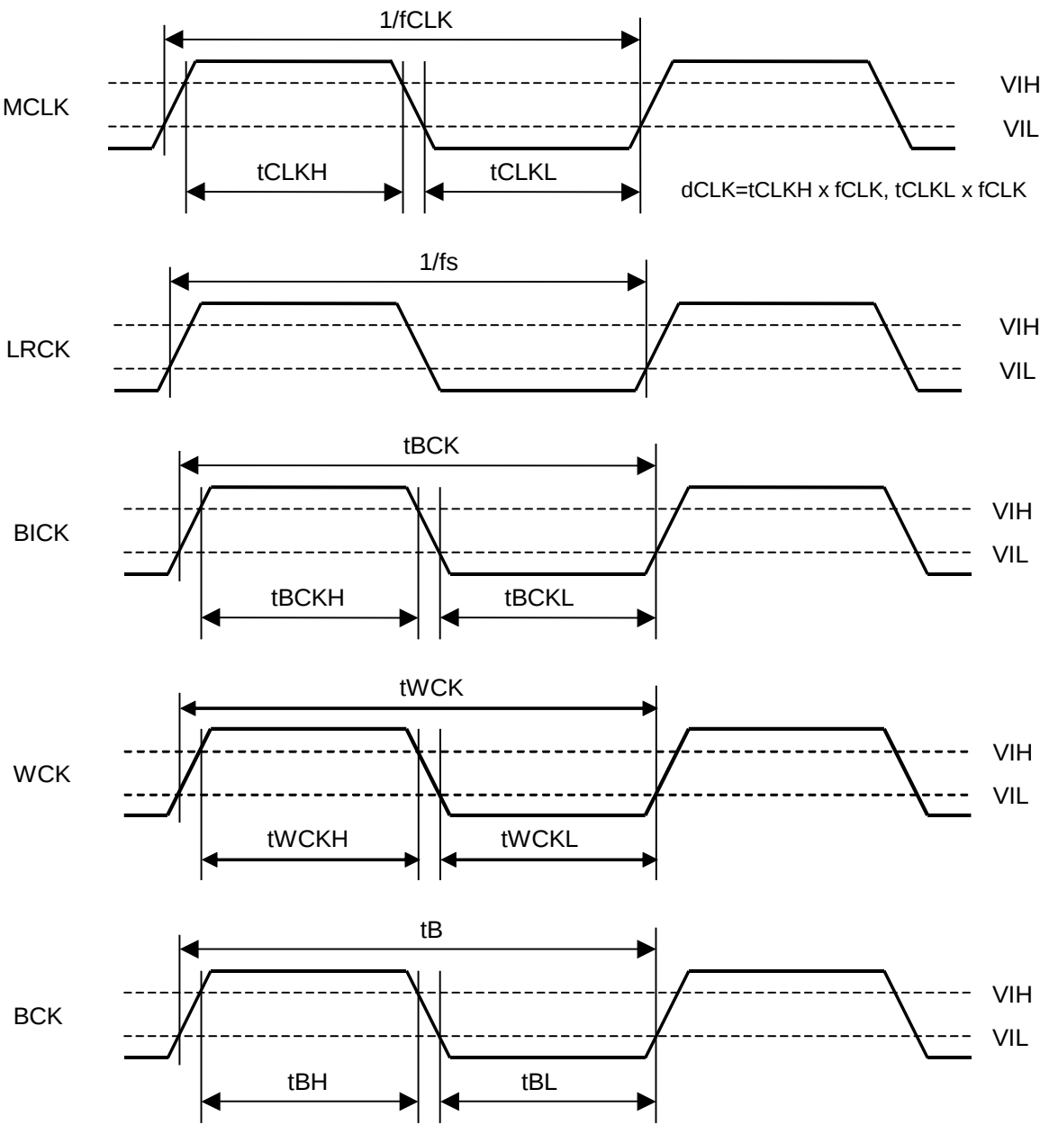
Clock Timing
