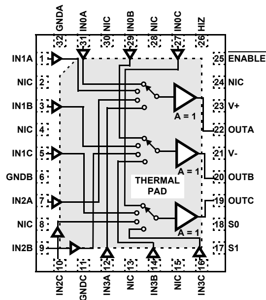
ISL59445 (32-LD QFN) TOP VIEW
