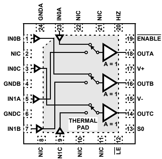
ISL59424 (24-LD QFN) TOP VIEW
