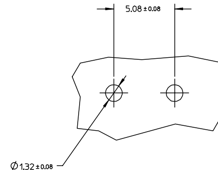
PRINTED CIRCUIT BOARD HOLE PATTERN
