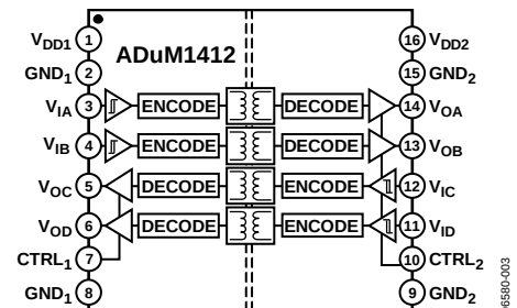
Figure 3. ADuM1412
