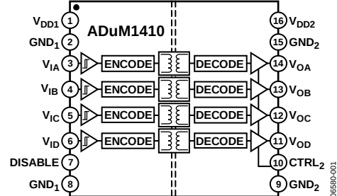
Figure 1. ADuM1410
