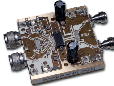
BLM7G22S-60PBG demoboard
