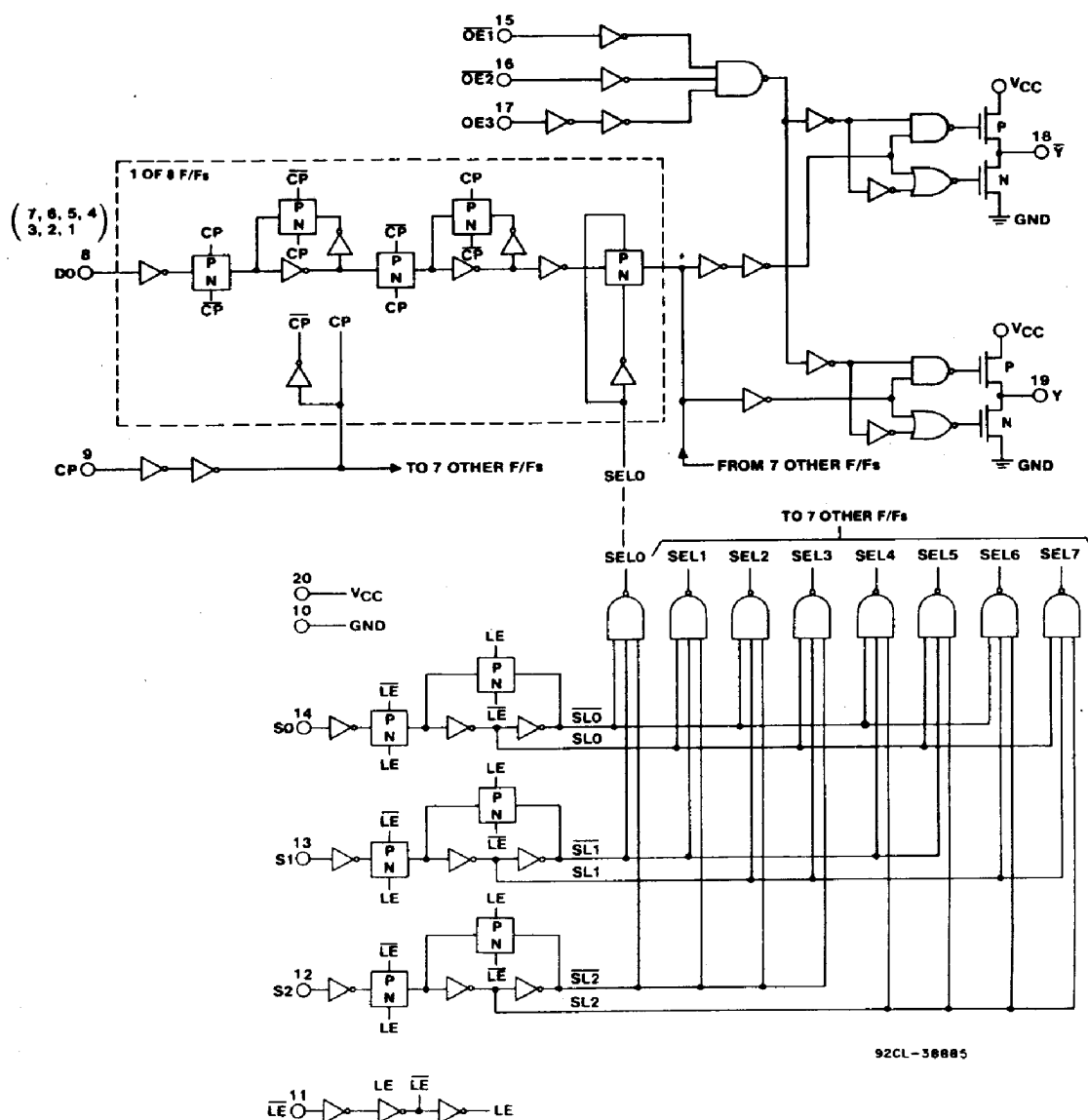
HC/HCT356 Logic Diagram
