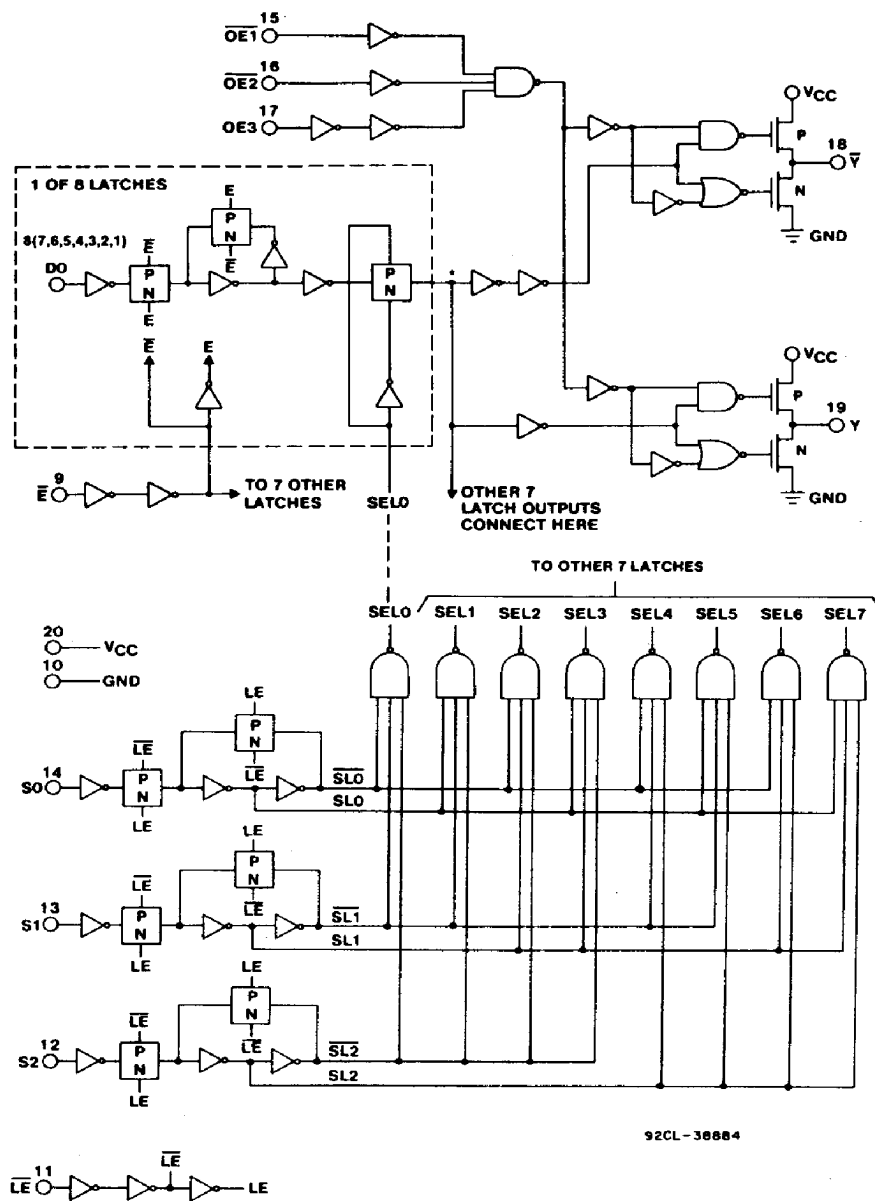
HC/HCT354 Logic Diagram
