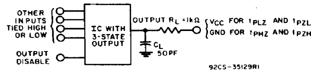
Fig. 2 — Three-state propagation delay test circuit.
