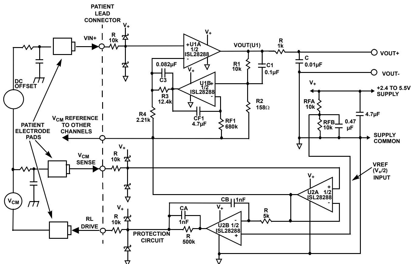
FIGURE 40. ECG AMPLIFIER
