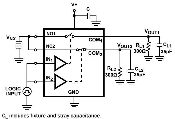
FIGURE 3B. TEST CIRCUIT (ISL5122 ONLY)
