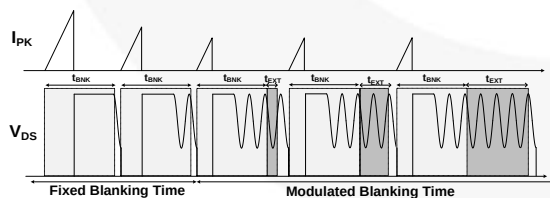
Figure 23. Frequency Fold-back Function
