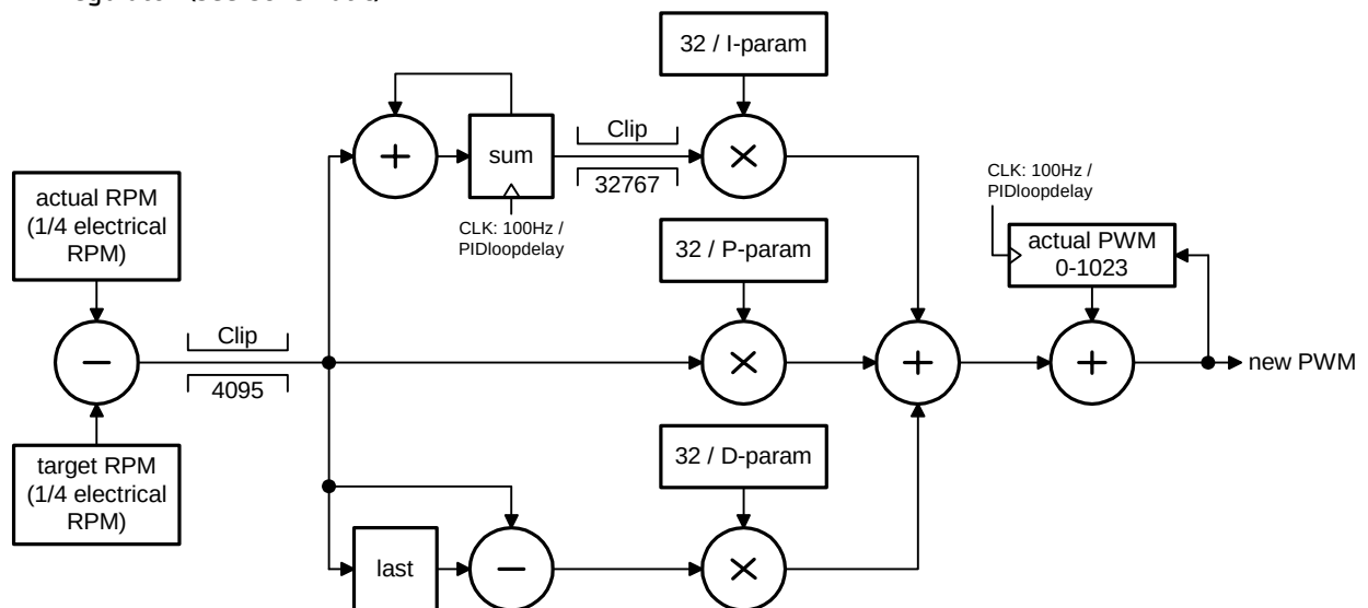
Figure 5.1: PID velocity regulator parameters
