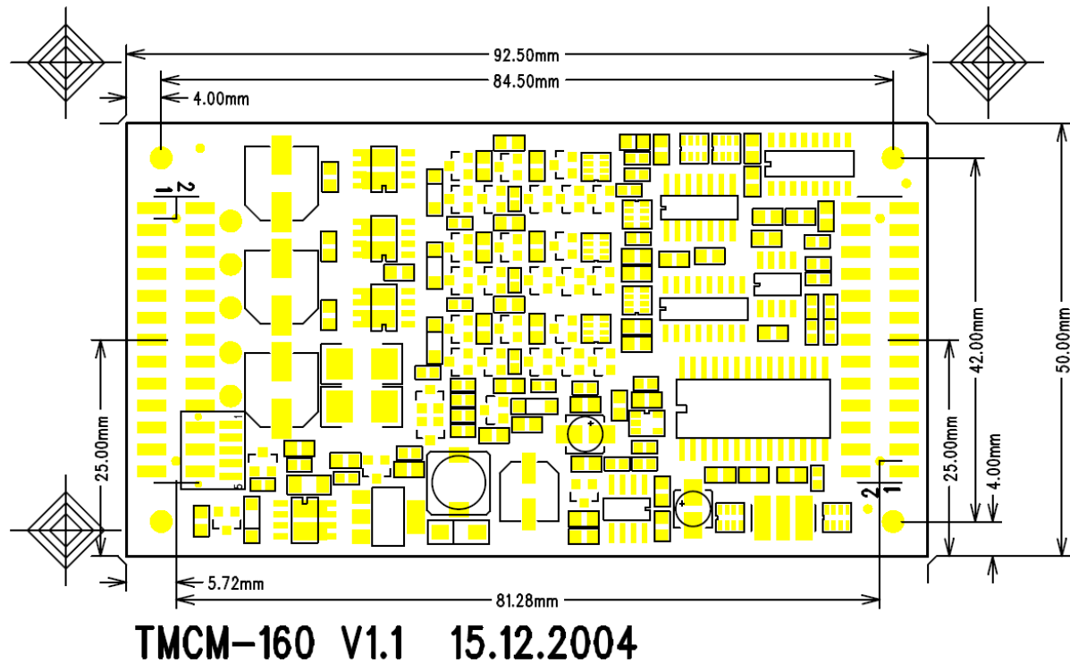
Figure 3.2: Dimensions
