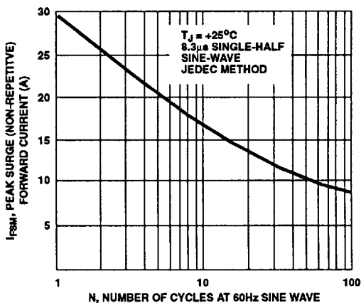
FIGURE 6. PEAK SURGE CAPABILITY vs NUMBER OF CYCLES
