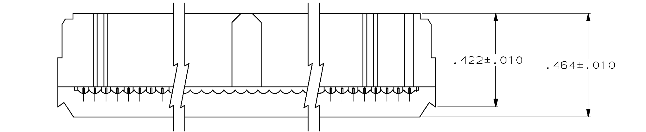
TERMINATED VIEW
