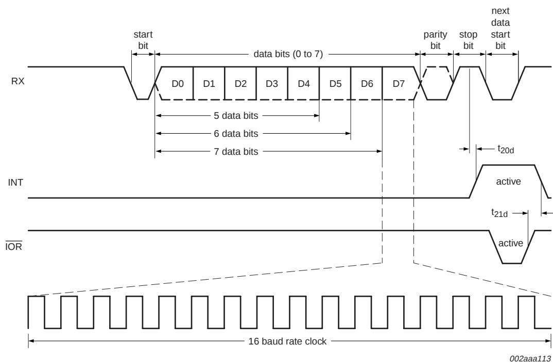
Fig 10. Receive timing
