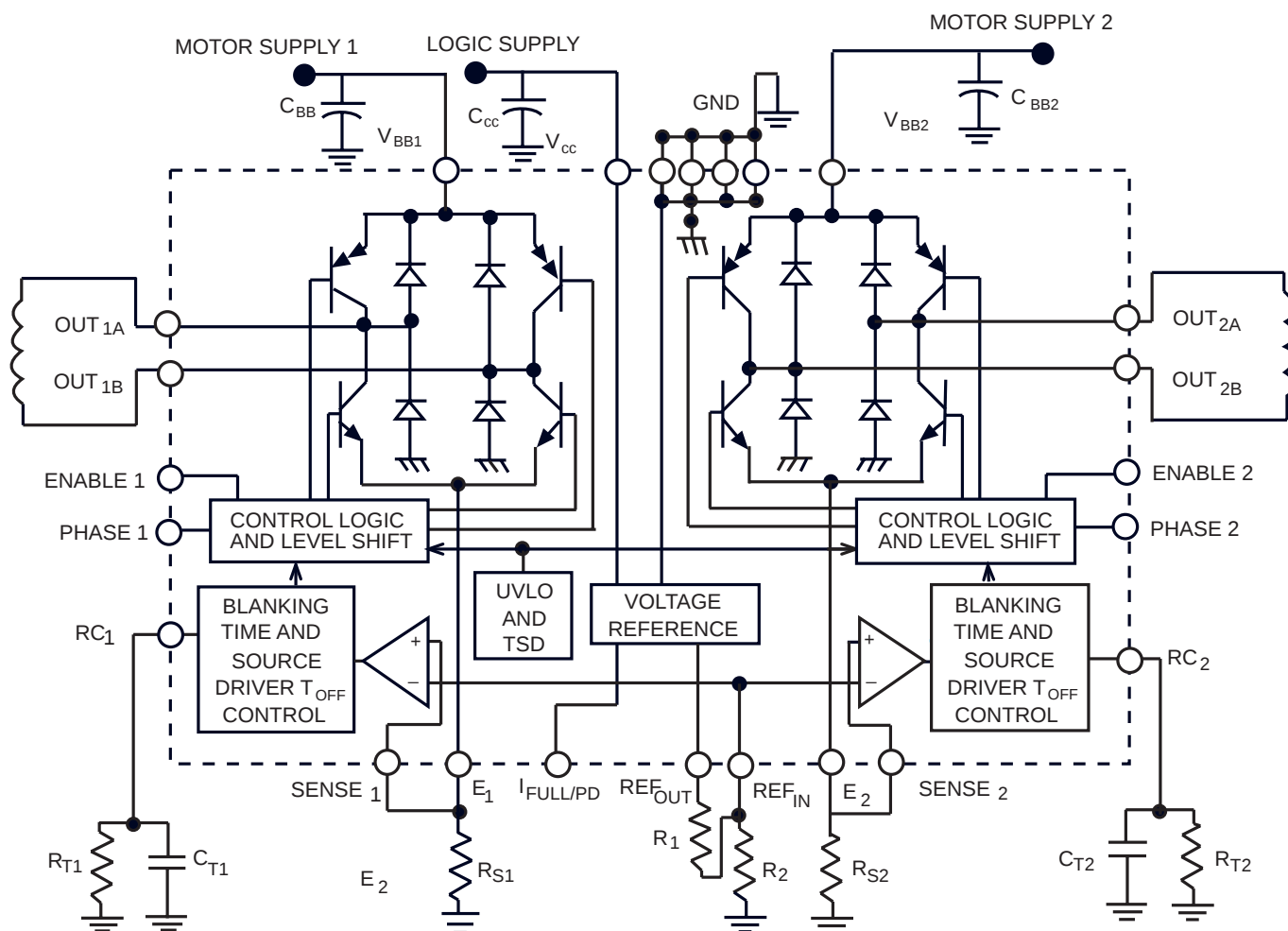
FUNCTIONAL BLOCK DIAGRAM AND TYPICAL BIPOLAR STEPPER MOTOR APPLICATION
