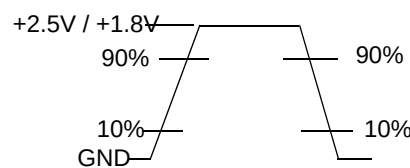
Figure 24. LVCMOS I/O Input Waveform
