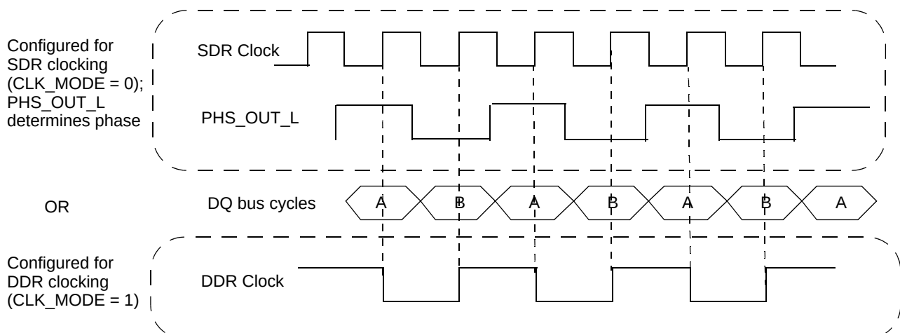
Figure 14. Ayama 20000 Clocks
