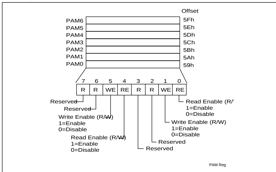
Figure 3. PAM Registers
