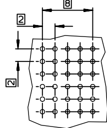
LAYOUT FOR P.C.B
