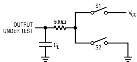
Figure 5. Driver Timing Test Load #2
