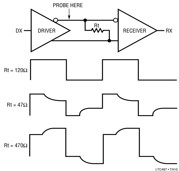
Figure 9. Termination Effects
