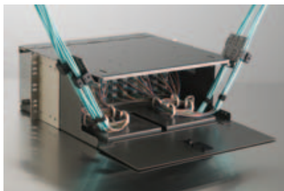
Close-up of PCH-04U Cable Entry with Panels Removed | Photo LAN587
