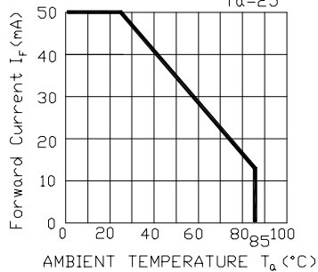
Forward Current Derating Curve T_a = 25^\circ
