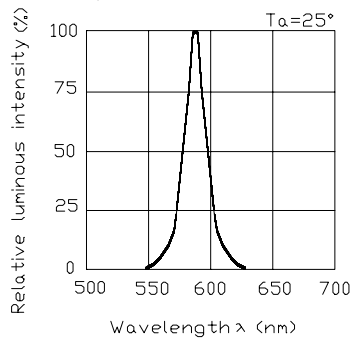
Spectrum Distribution T_a = 25^\circ
