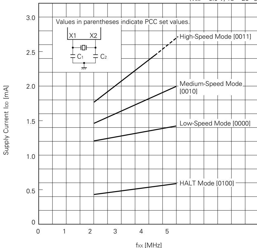
I_{DD} vs. f_{XX} Characteristic Examples (Ceramic Oscillation)
