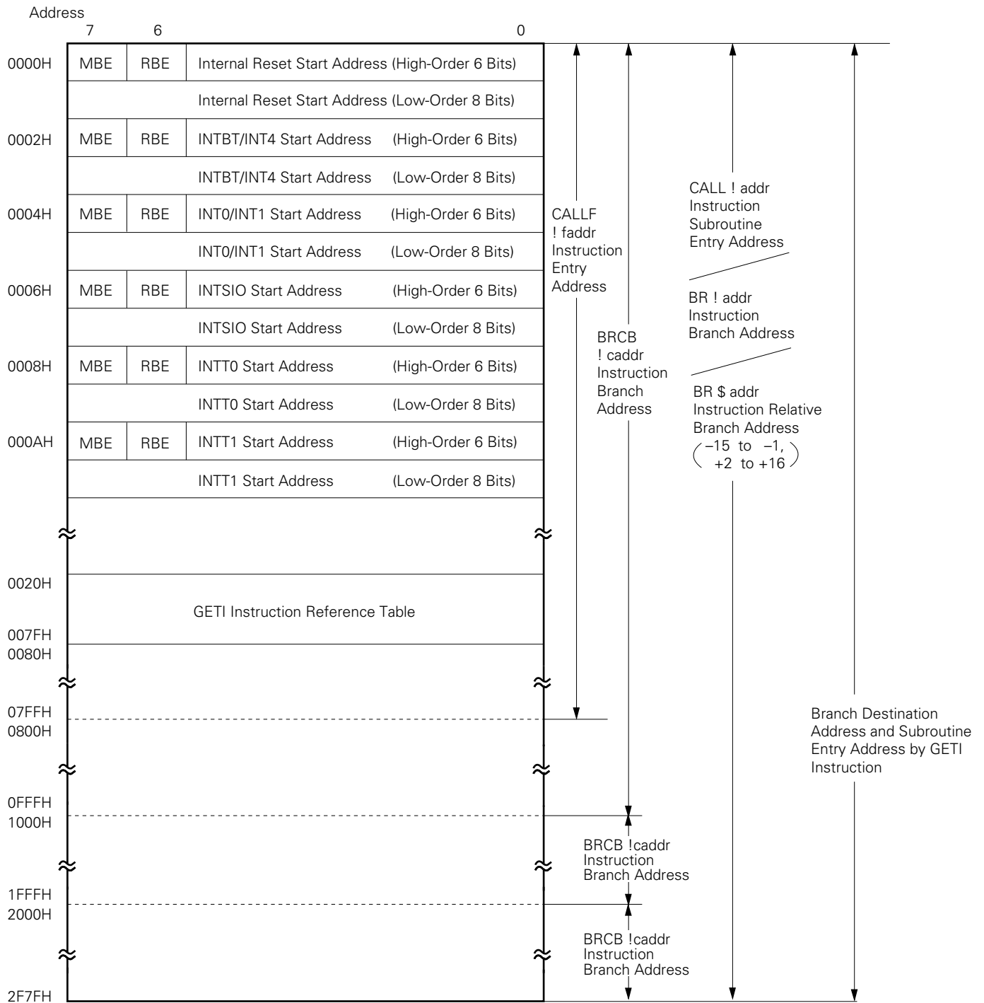
Fig. 4-2 Program Memory Map ( \mu PD75112F)
