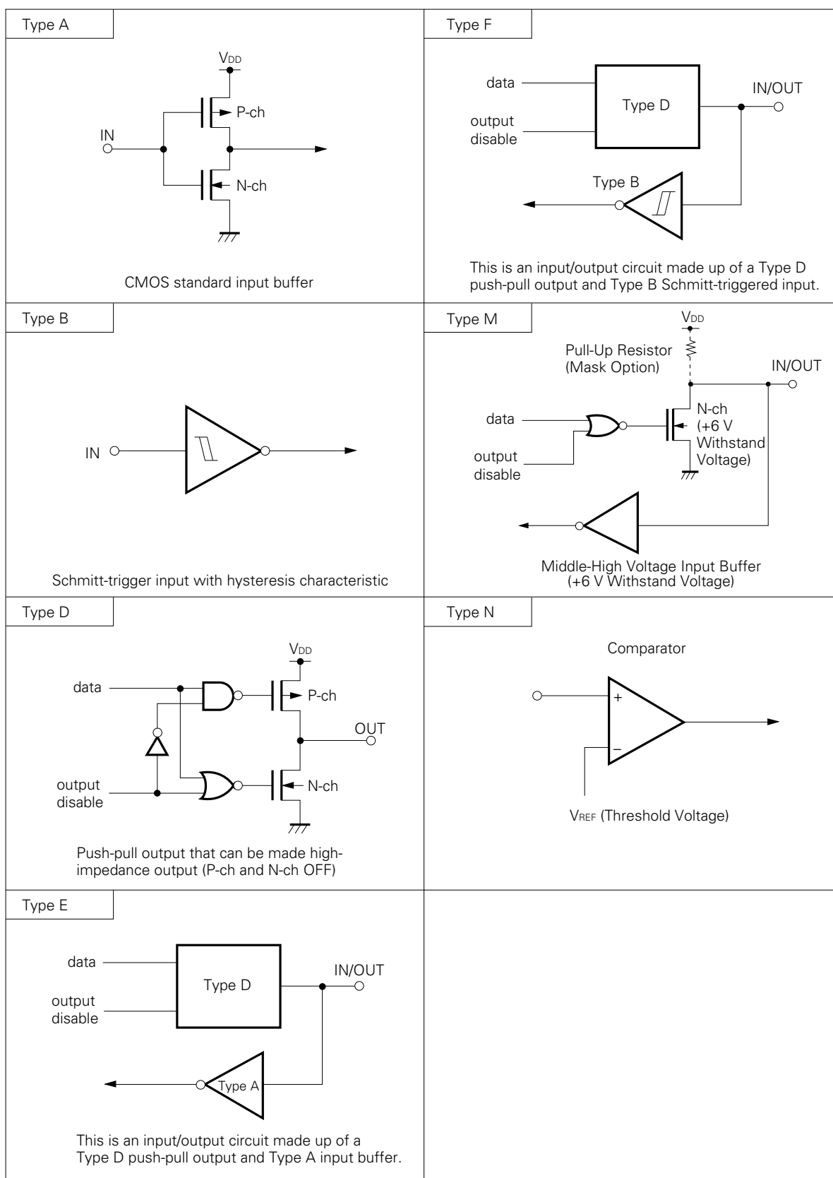
Fig. 3-1 Pin Input/Output Circuit List
