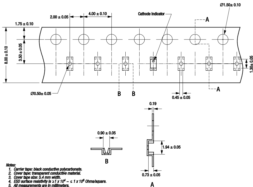
Figure 7. SC-79 Tape and Reel Dimensions
