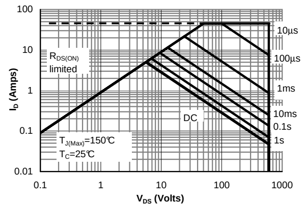
Figure 12: Maximum Forward Biased Safe Operating Area for AOWF11S60 (Note F)
