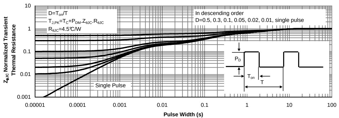
Figure 16: Normalized Maximum Transient Thermal Impedance for AOWF11S60 (Note F)
