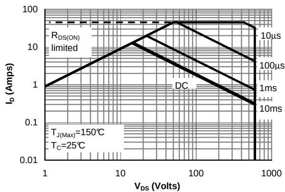
Figure 11: Maximum Forward Biased Safe Operating Area for AOW11S60 (Note F)
