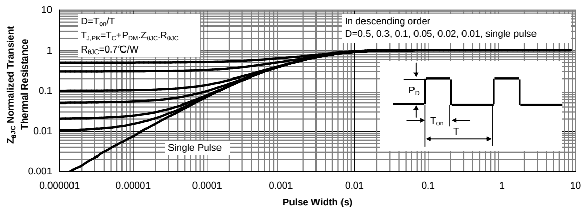
Figure 15: Normalized Maximum Transient Thermal Impedance for AOW11S60 (Note F)
