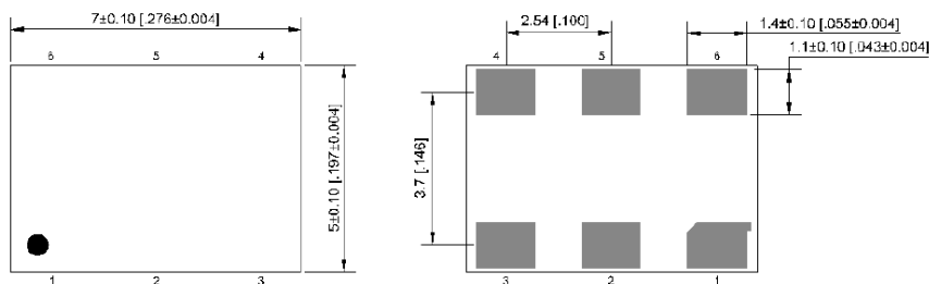
External Dimensions
