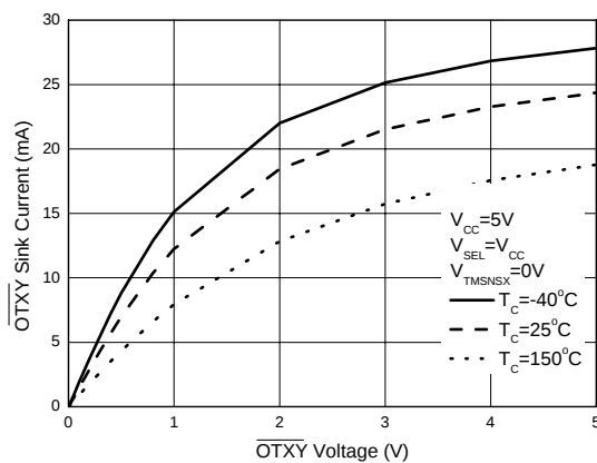
Figure 10. Open-drain \overline{\text{OTXY}} Output Sink Current vs. \overline{\text{OTXY}} Voltage
