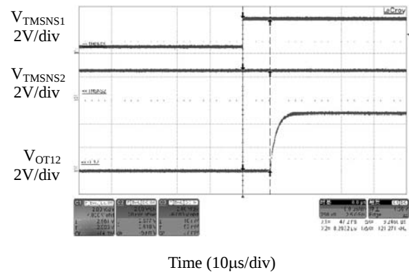
Figure 11. Deglitch time to OT High ( V_{SEL} = V_{CC} ) (Conditions: V_{CC} = 5\text{V} , V_{TMSNS1} = 0.5\text{V} to 3\text{V} , V_{TMSNS2} = 2.5\text{V} )
