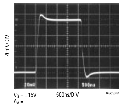
±15V Small-Signal Response
