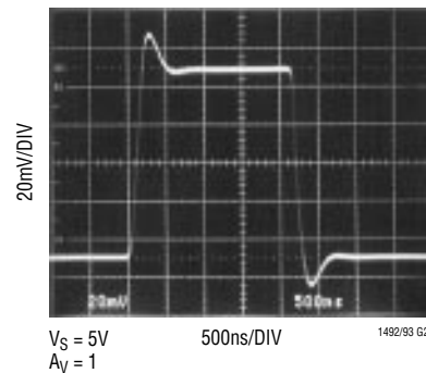
5V Small-Signal Response
