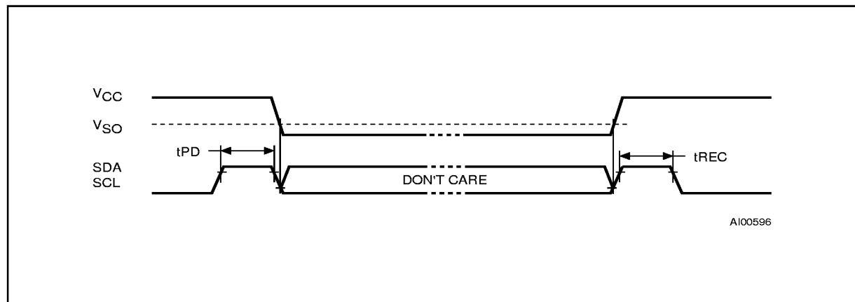
Figure 5. Power Down/Up Mode AC Waveforms
