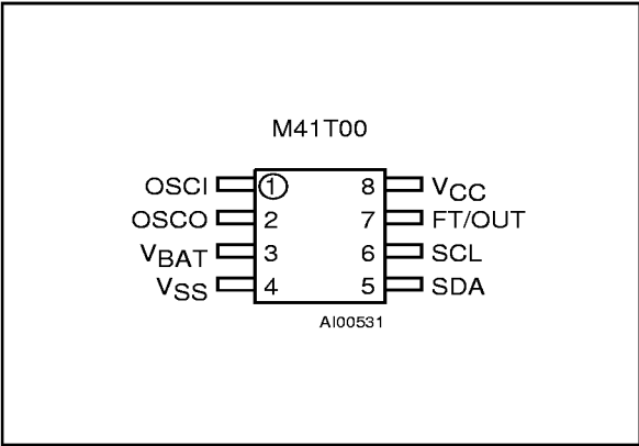
Figure 2. SOIC Pin Connections
