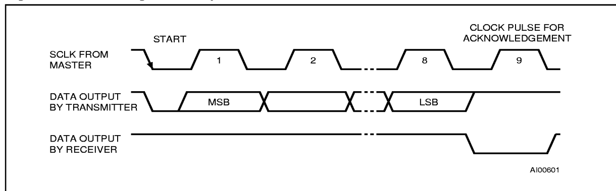
Figure 7. Acknowledgement Sequence
