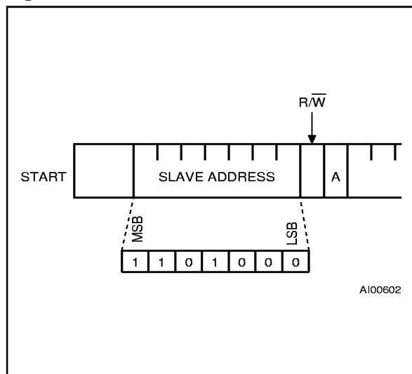
Figure 9. Slave Address Location
