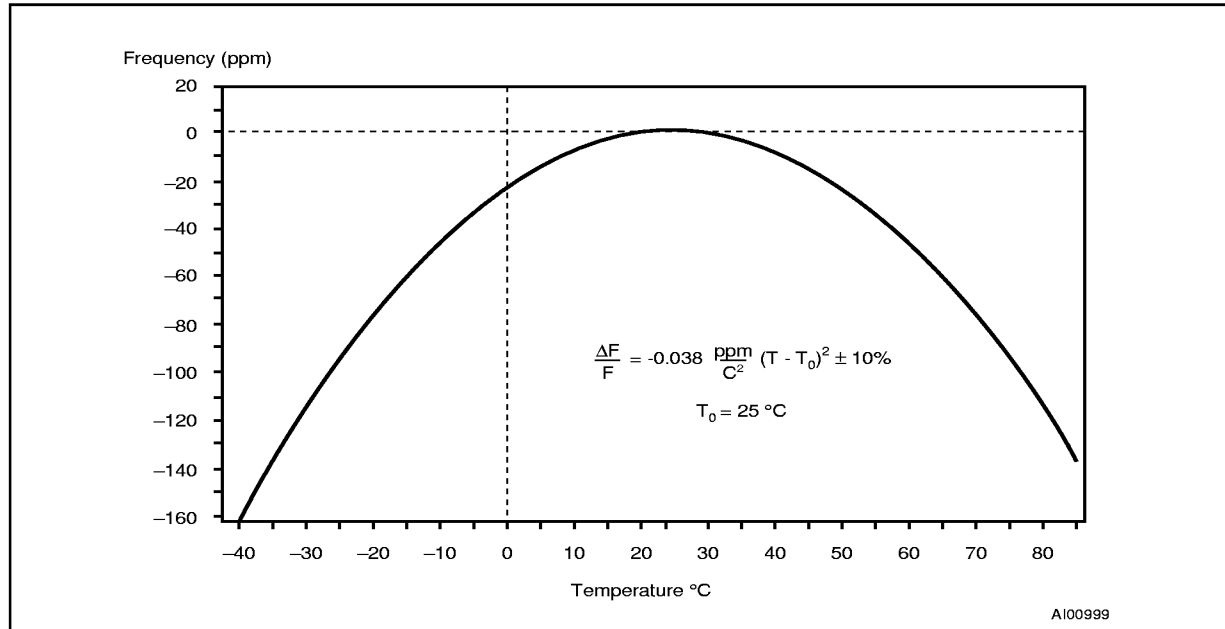
Figure 14. Crystal Accuracy Across Temperature
