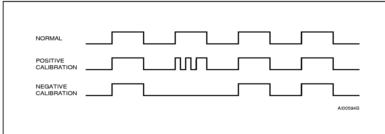
Figure 13. Clock Calibration
