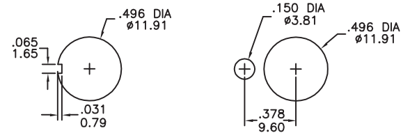
15/32 INCH BUSHING
