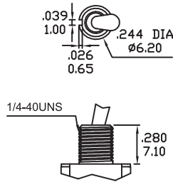
B8 METRIC
