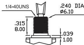
BA THD For T6
