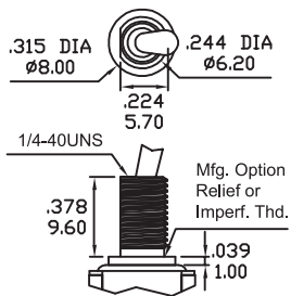
BA THD For T6
