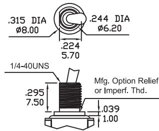
B9 SPLASH-PROOF
