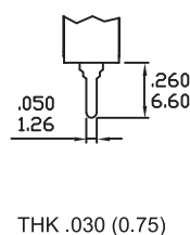
M2 PC THRU-HOLE
