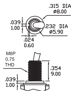
B8 METRIC
