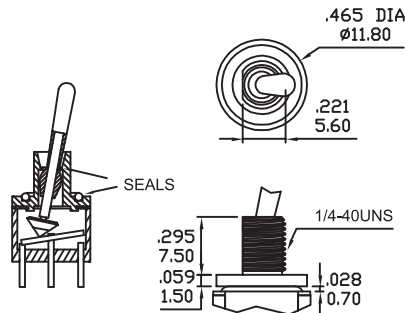
B9 SPLASH-PROOF
