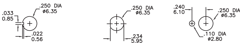
1/4 INCH BUSHING
