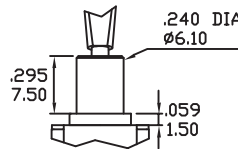
BB NON-THD For T6
