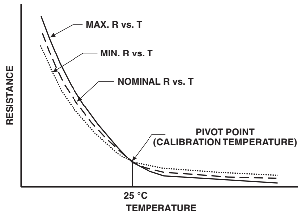
FIGURE 2 POINT MATCH TOLERANCES VS. TEMPERATURE
