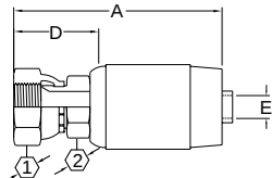
SAE 37° (JIC) swivel FJ9782
