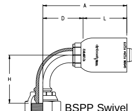
BSPP Swivel 90° Elbow
