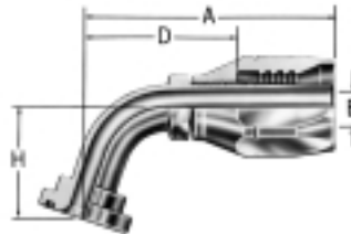
67 1/2° split flange FC9118-/FC7811- Code 61 SAE J518 FC7984-/FJ9034- Code 62 SAE J518
