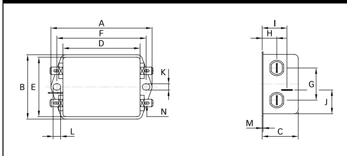
Connection style -06, 1 and 3 A types
