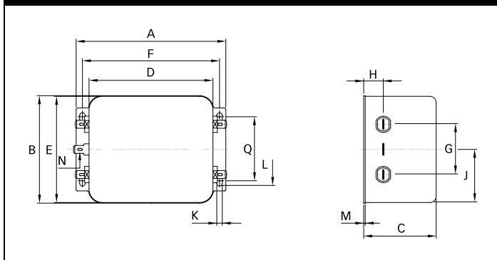
Connection style -06, 16 A types
