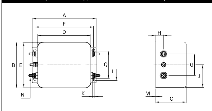
Connection style -08, 16 A types (same dimensions as style -06)
