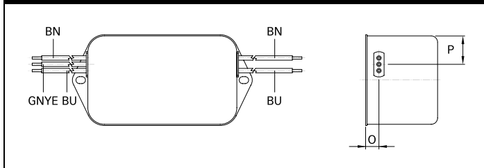
Connection style -07, 6 to 12 A types (same dimensions as style -06)
