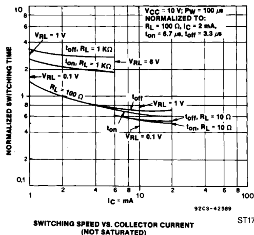
2. Switching Speed vs. Collector Current (Not Saturated)
