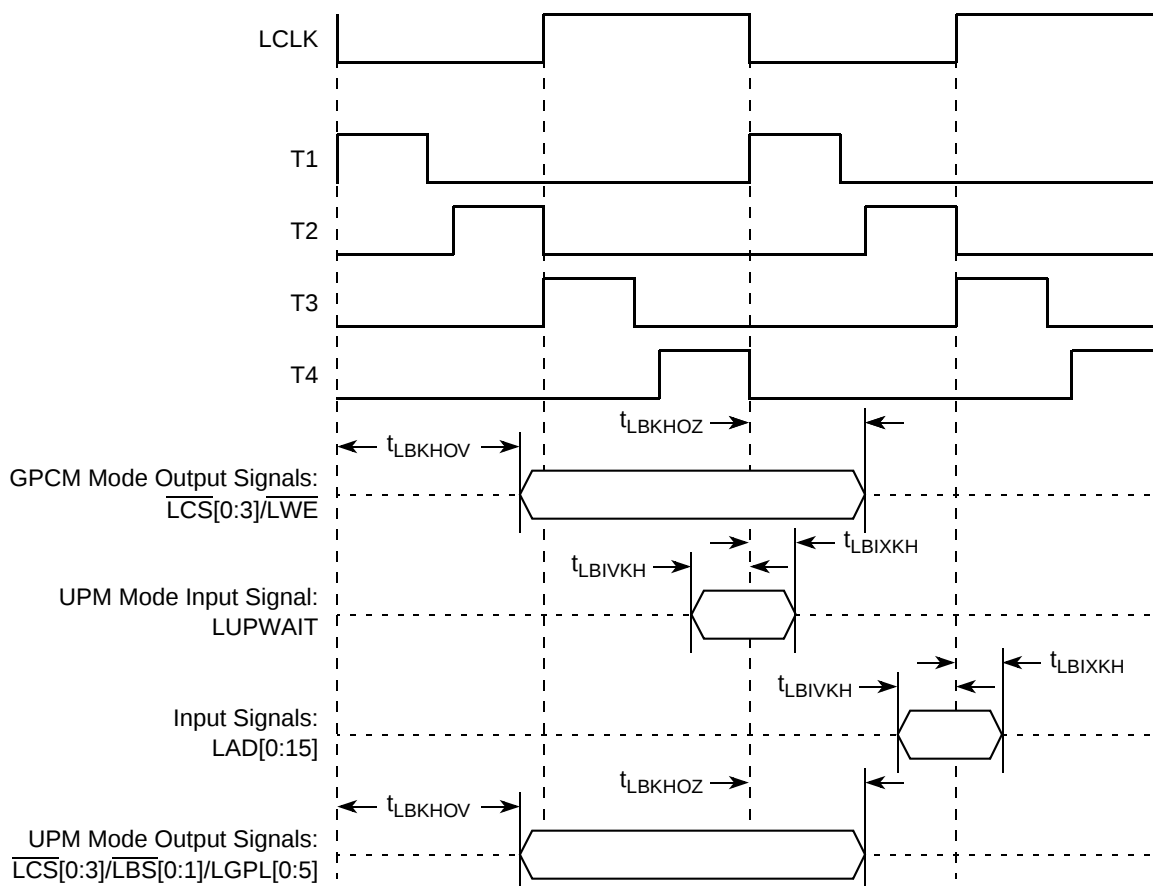
Figure 39. Local Bus Signals, GPCM/UPM Signals for \text{LCRR}[\text{CLKDIV}] = 4
