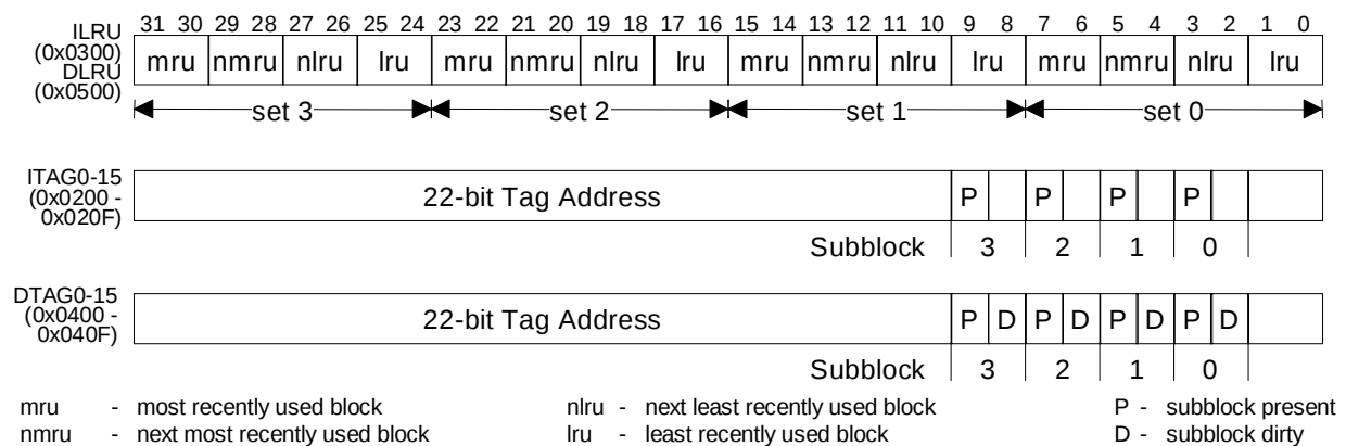
Figure 17. Cache Registers
