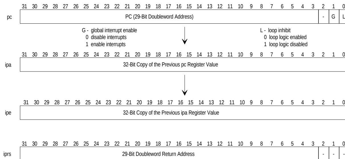
Figure 30. Pipeline Registers
