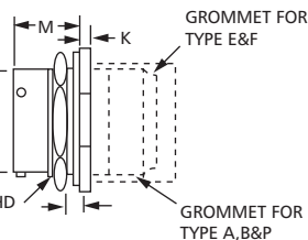
CRIMP KPSE07/MS3114
