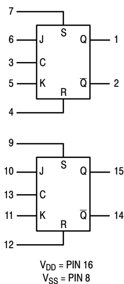
BLOCK DIAGRAM
