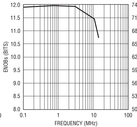
ENOBs and SINAD vs Input Sinewave Frequency for Differential Input Signals
