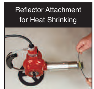
Reflector Attachment for Heat Shrinking
