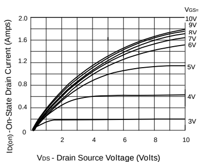
Saturation Characteristics
