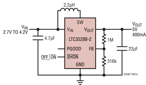
Li-Ion to 5V
