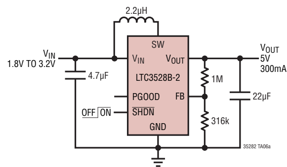
2 Cell to 5V
