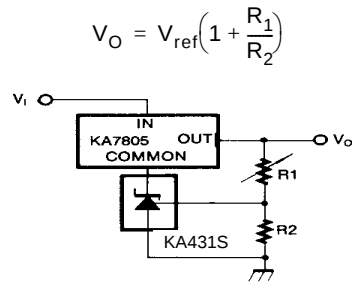
Figure 14. Output Control for Three-Termianl Fixed Regulator
