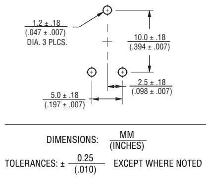
SUGGESTED PWB LAYOUT
