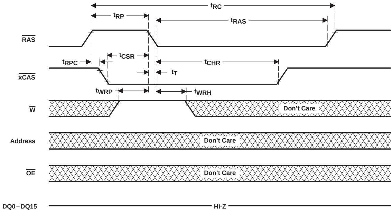
Figure 16. Automatic (xCBR) Refresh-Cycle Timing
