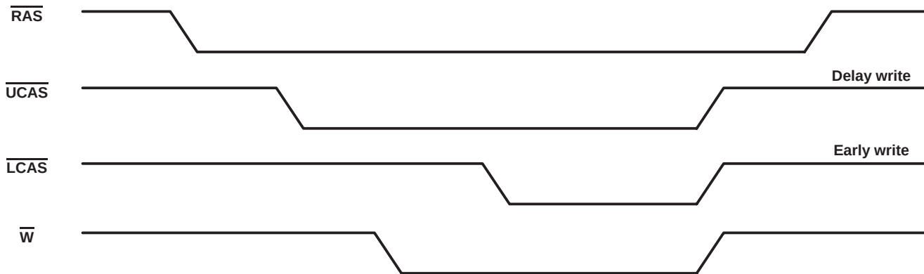
Figure 1. Illegal Dual-xCAS Operation
