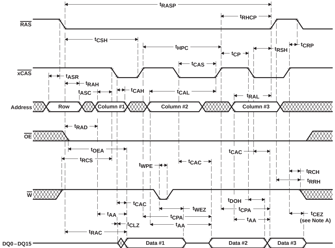
Figure 9. EDO Read-Cycle Timing With \overline{W} Control
