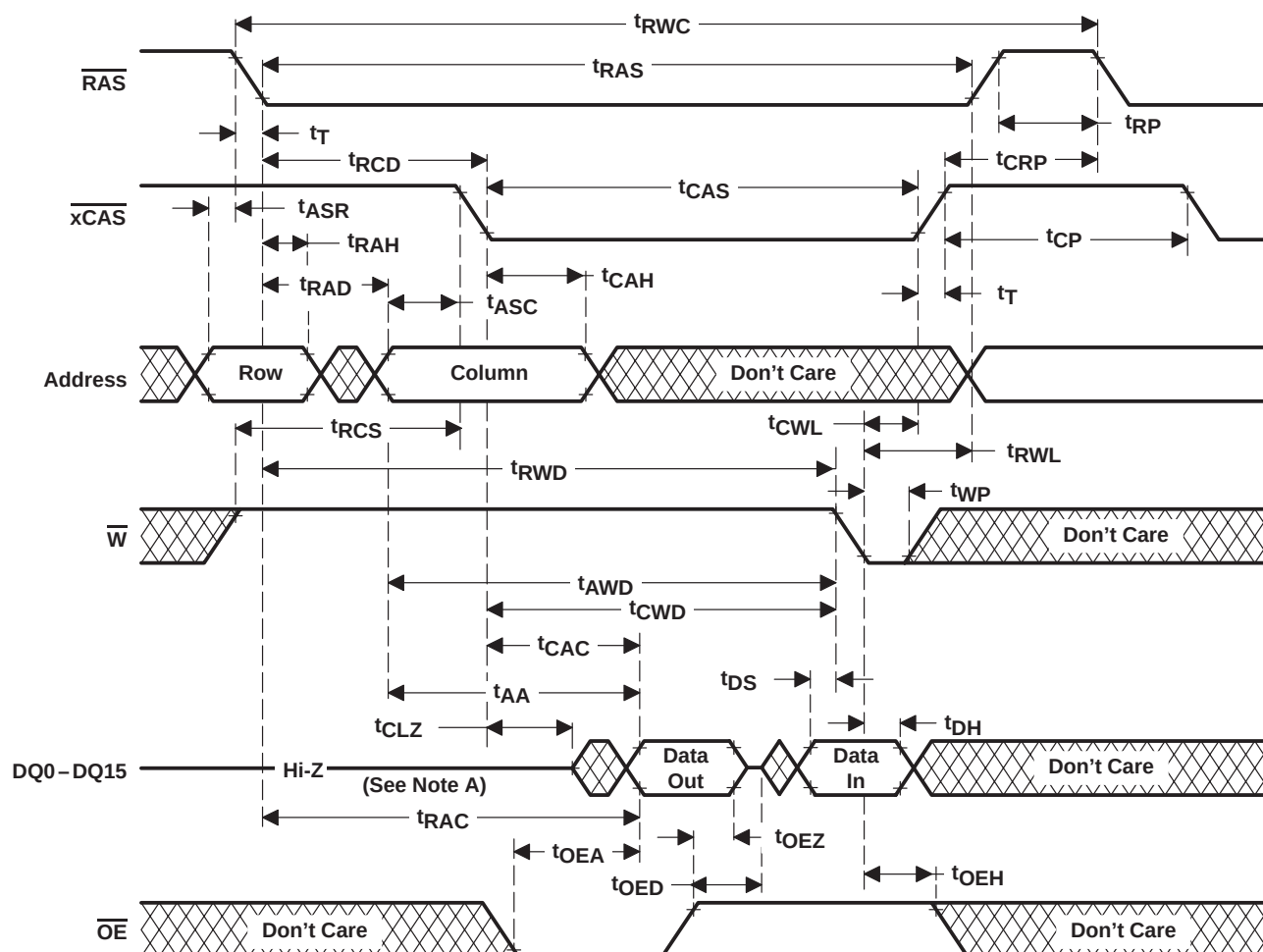
Figure 6. Read-Write-Cycle Timing
