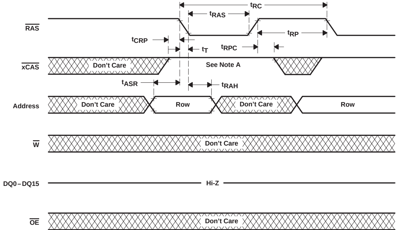
Figure 13. \overline{\text{RAS}} -Only Refresh-Cycle Timing
