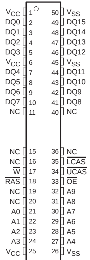
DGE PACKAGE (TOP VIEW)
